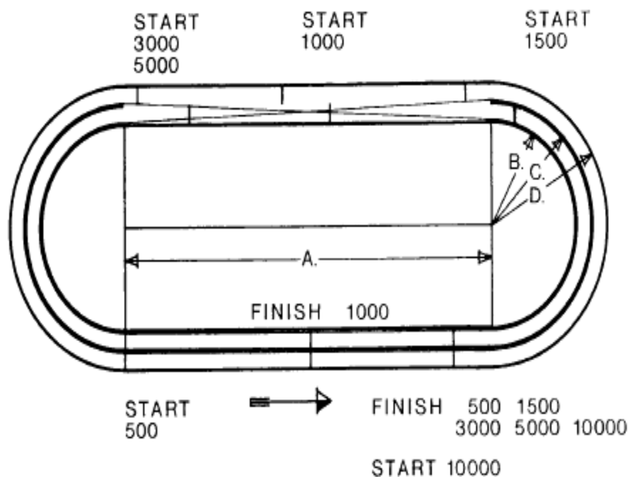
Diagram of a Standard Speed Skating Track
